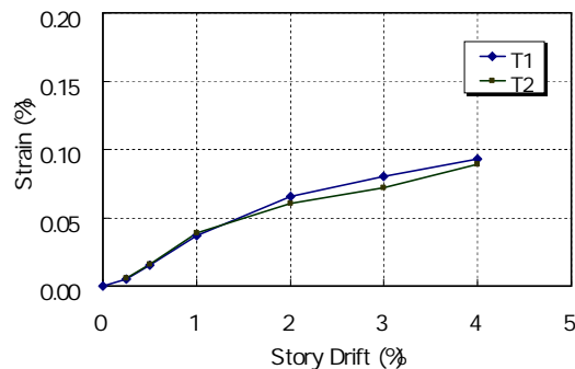
Figure 13. Strain of the U-shaped steel box
