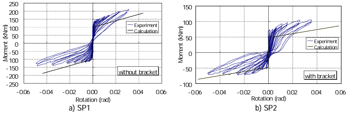
Figure 9. Moment-Rotation Relationship
