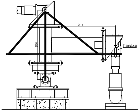
Figure 5. Measurement system of story drift
