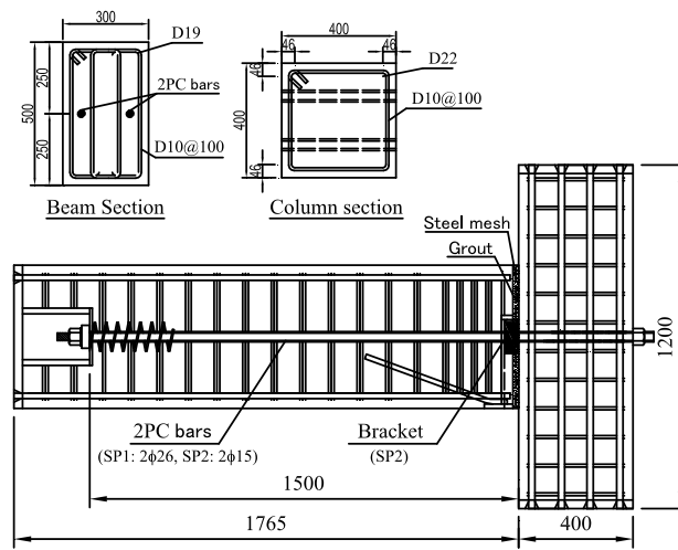
Figure 1. Reinforcement details of specimens SP1, SP2
