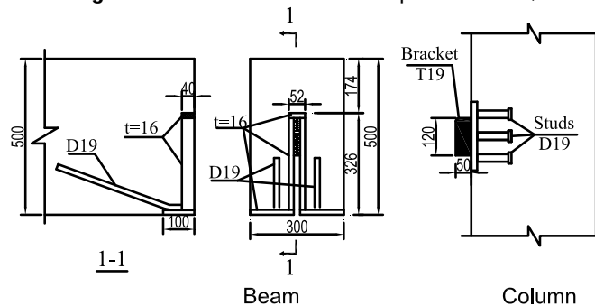
Figure 2. Details of the shear bracket, SP2
