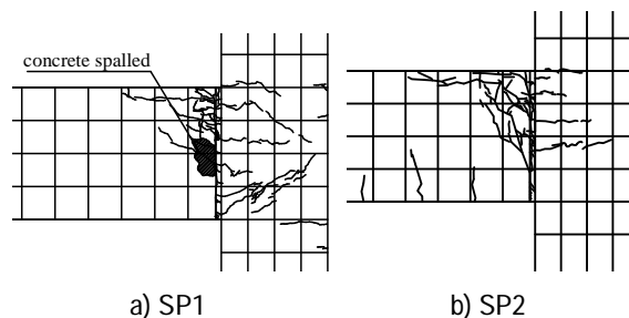
Figure 6. Crack pattern of specimens after 4% drift
