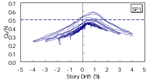
Figure 11. Variation of beam shear force/PC force ratio
