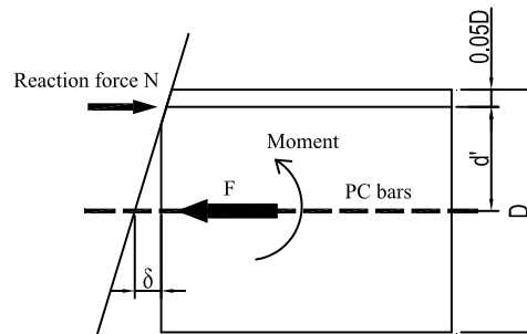
Figure 8. Determination of d'
