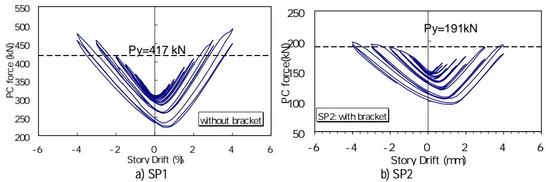
Figure 12. PC force – Story drift relationship
